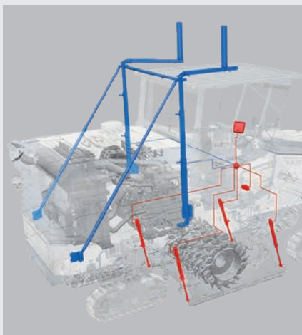
3D leveling / laser leveling
