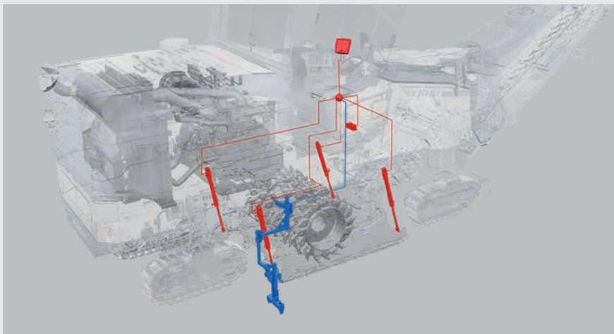
Sonic-Ski sensor
